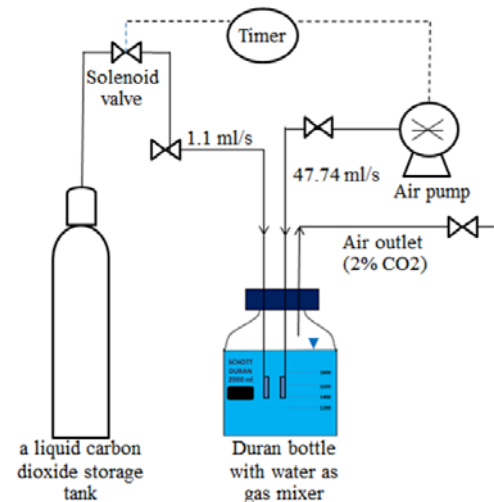
Fig. 2. Diagram of external \text{CO}_2 mixing device in this experiment.
